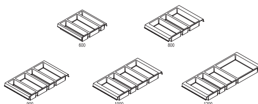
Pull-out organisation concept anthracite, height: 100 mm, fits pull-out depth of 500 mm, side depth: 561 mm
