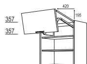
Wall unit, folding/lifting door 1 folding/lifting door, 2 original fronts, 2 shelves
