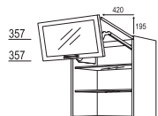
Wall unit, folding/lifting door 1 folding/lifting door, 1 top original front, 1 bottom framed glass front, clear glass No. 01, 2 glass shelves, glass variations for a surcharge: No. 02 / 39
