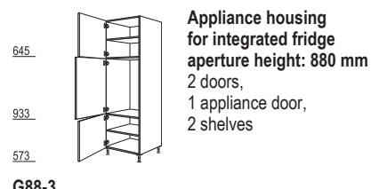
Appliance housing for integrated fridge aperture height: 880 mm 2 doors, 1 appliance door, 2 shelves
