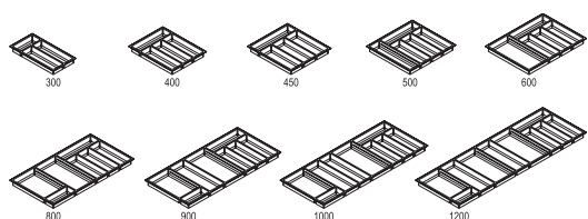
Universal organiser Alu profile with 4 dividers for individualised divisions, height: 125 mm, fits pull-out depth of 500 mm, side depth: 561 mm, 1 alu profile of 600 mm width, 2 alu profiles of 800 up to 900 mm width, 3 alu profiles of 1000 up to 1200 mm width
