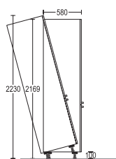
Tall unit height H-1 XL
